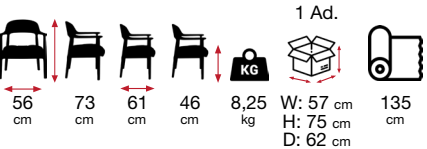
CEYLAN [CYM 01] Metal
